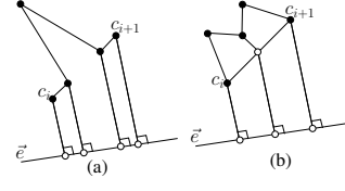
Fig. 23: \alpha_i has four edges.
